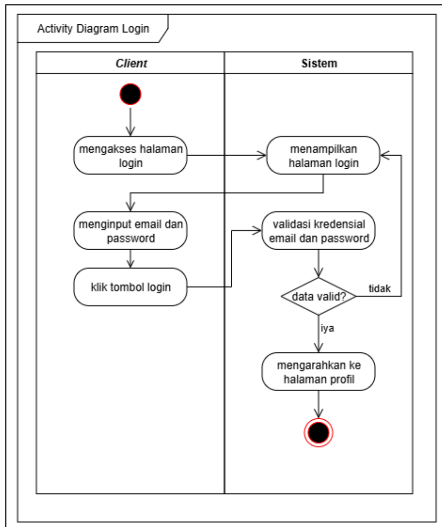
Gambar III.3 Activity Diagram Client Melakukan Login
