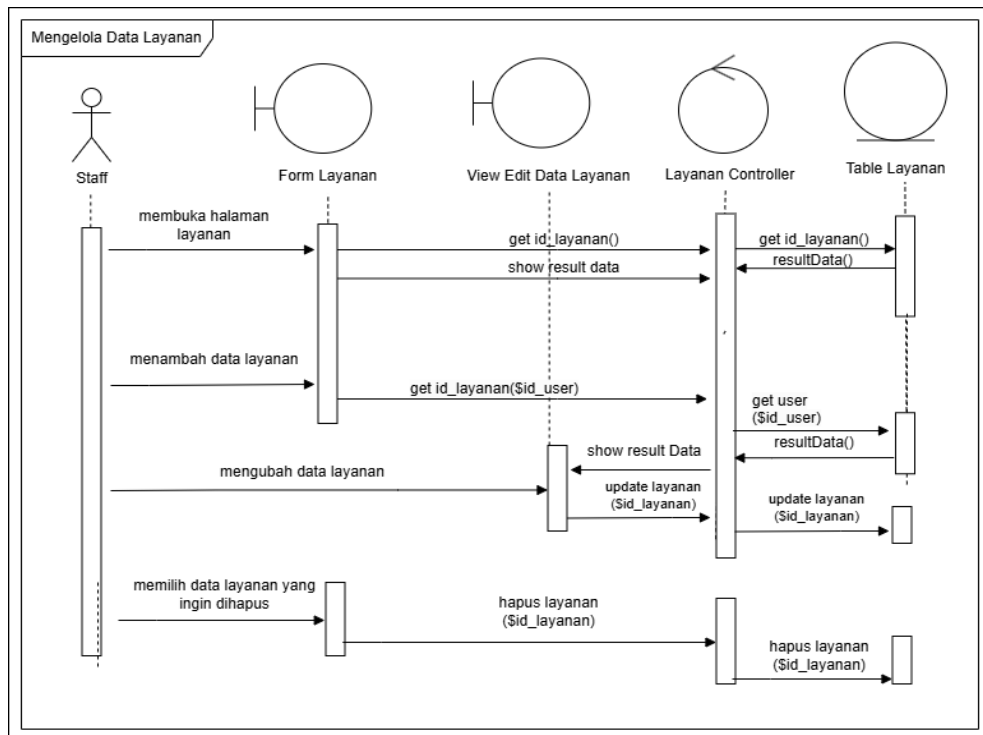
Gambar III.37 Sequence Diagram Staff Mengelola Data Layanan
