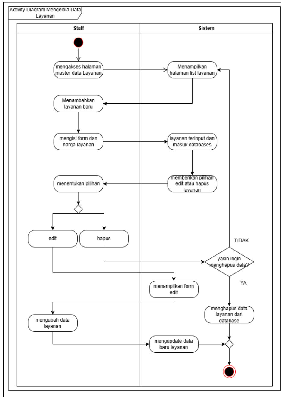
Gambar III.15 Activity Diagram Staff Mengelola Data Layanan
