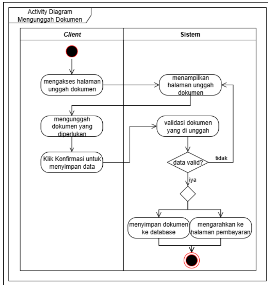
Gambar III.6 Activity Diagram Client Mengunggah Dokumen
