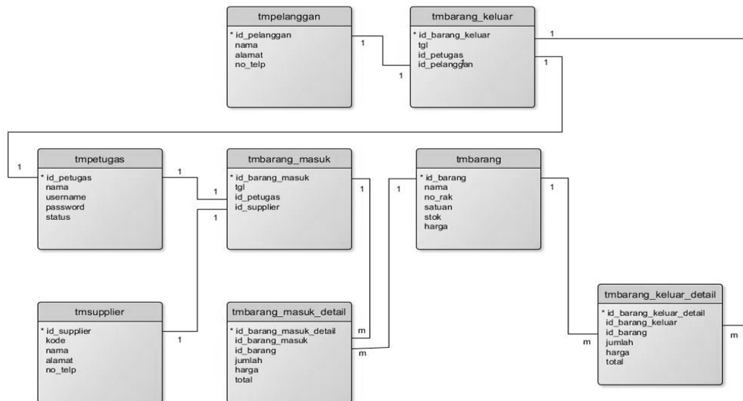
Gambar II.3 Contoh Logical Record Structure (LRS)
