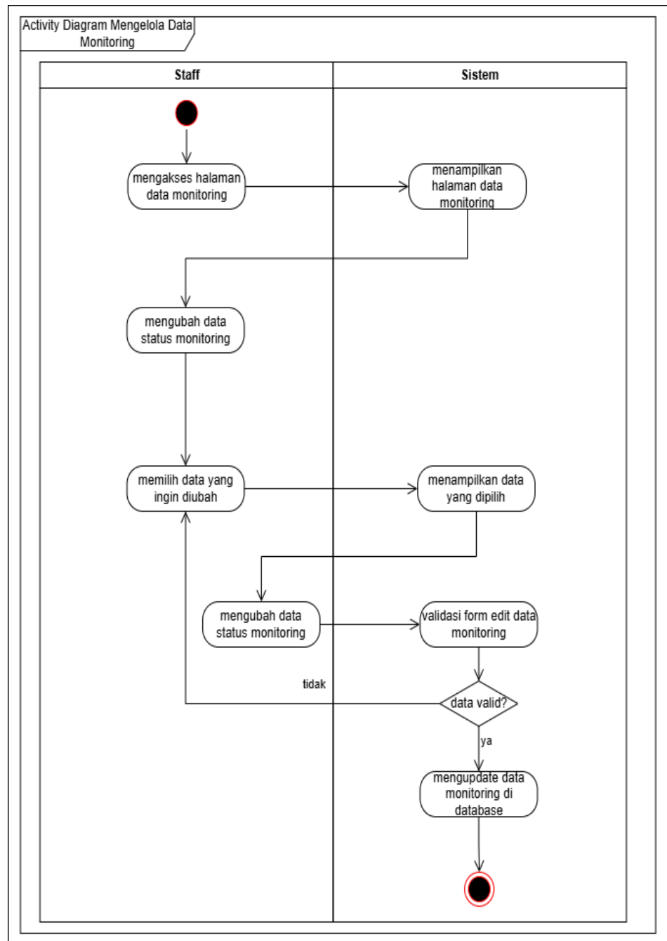
Gambar III.17 Activity Diagram Staff Mengelola Data Monitoring
