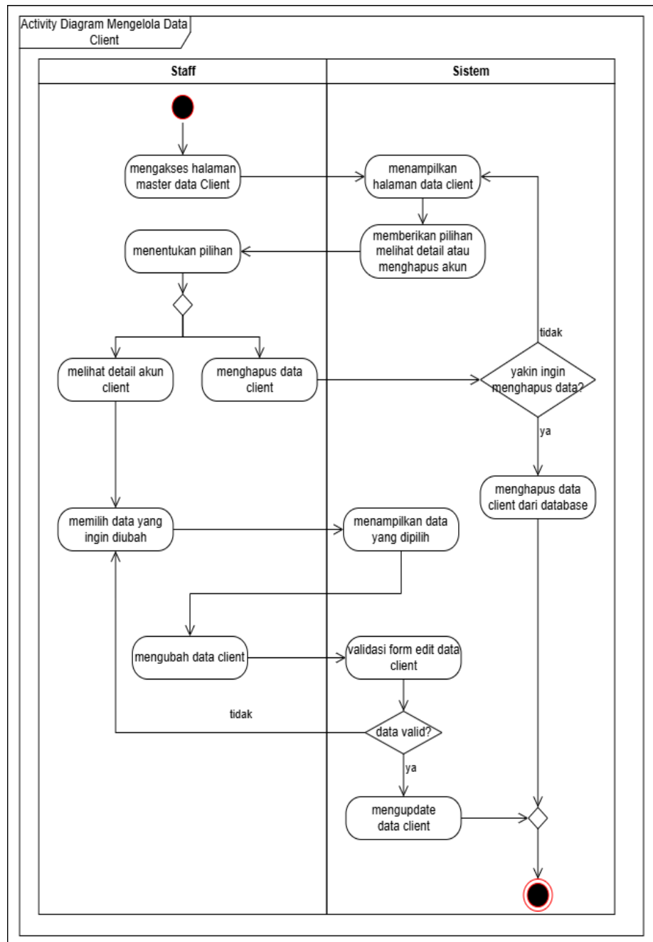
Gambar III.13 Activity Diagram Staff Mengelola Data Client
