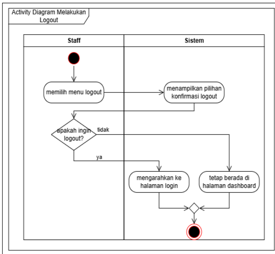
Gambar III.19 Activity Diagram Staff Melakukan Logout
