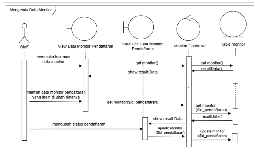
Gambar III.39 Sequence Diagram Staff Mengelola Data Monitoring
