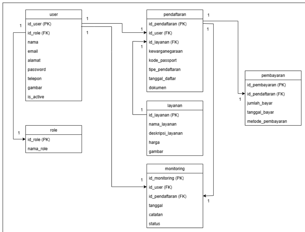
Gambar III.21 Logical Record Structure
