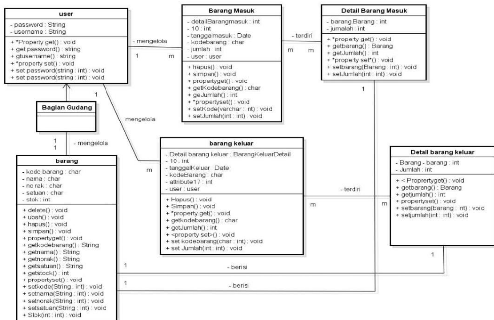
Gambar II.7 Contoh Class Diagram
