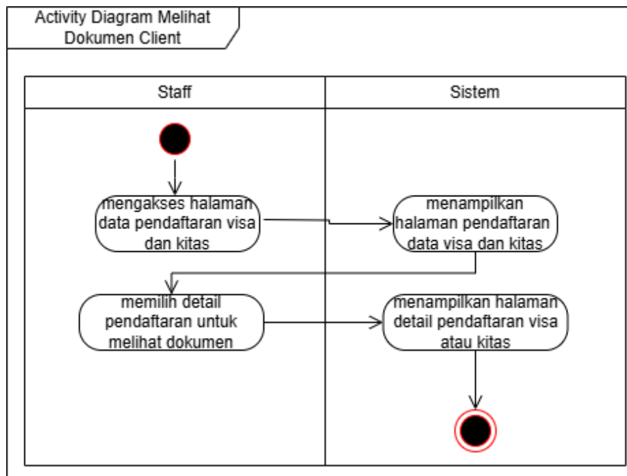
Gambar III.14 Activity Diagram Staff Melihat Dokumen Client
