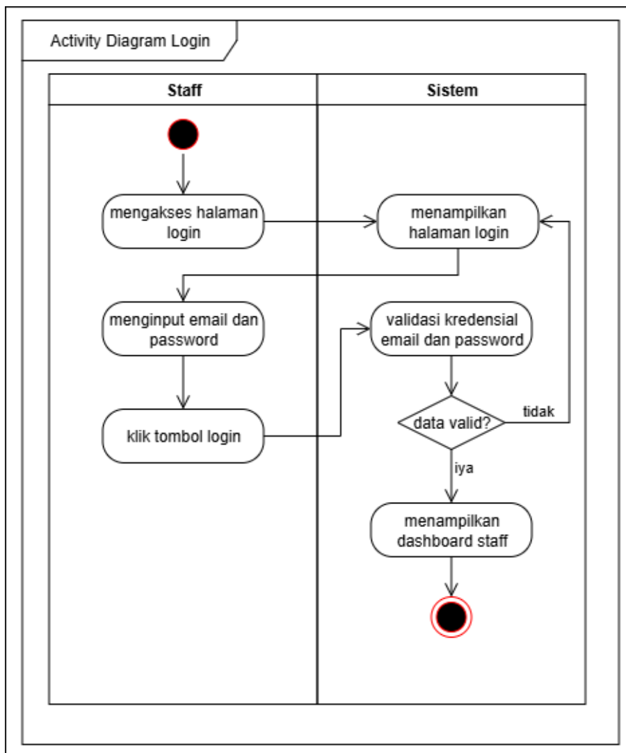
Gambar III.10 Activity Diagram Staff Melakukan Login
