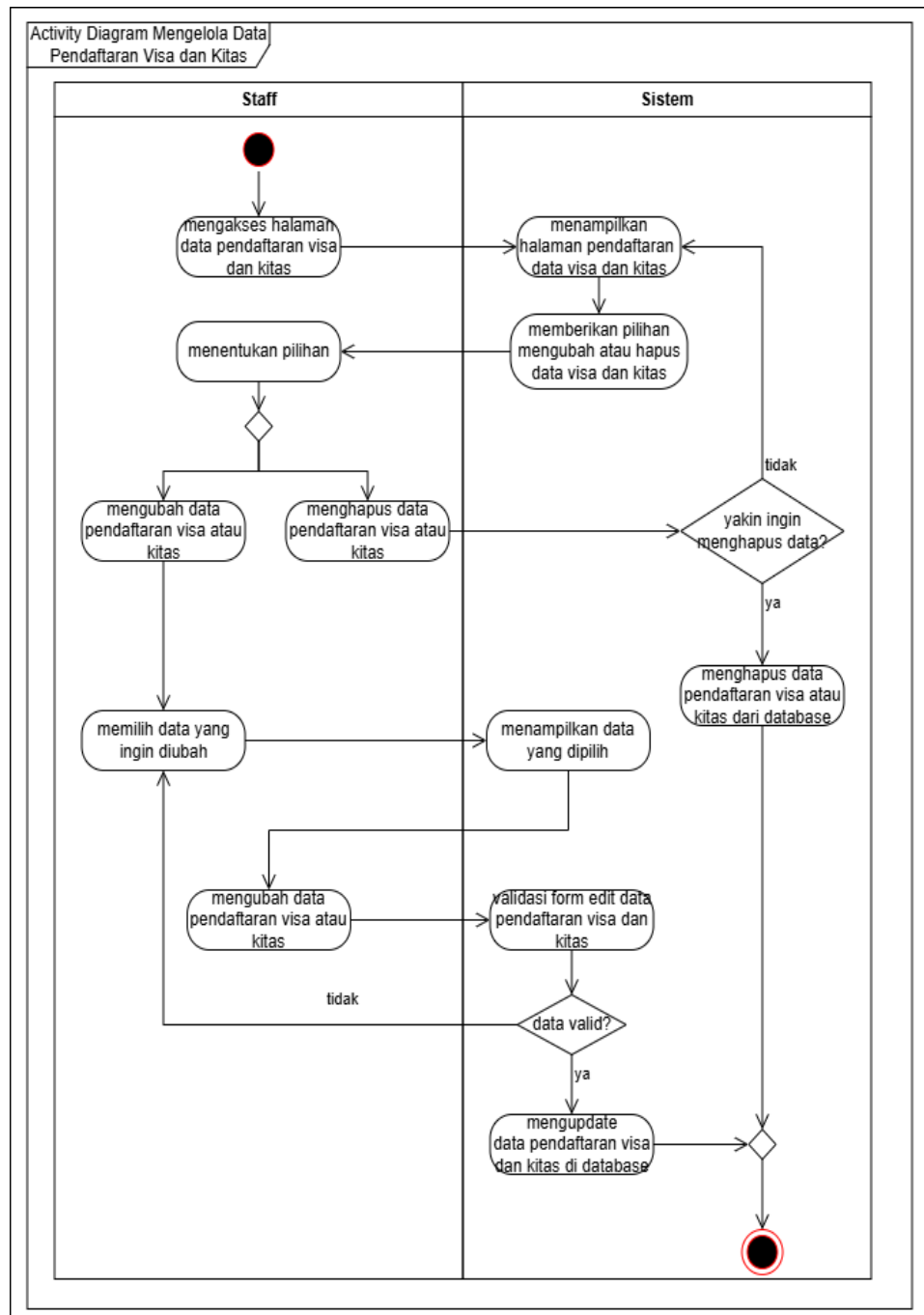
Gambar III.12 Activity Diagram Staff Mengelola Data Pendaftaran
