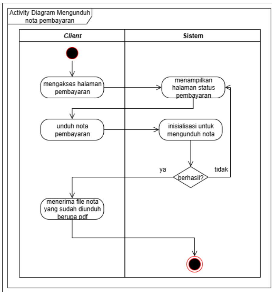
Gambar III.8 Activity Diagram Client Mengunduh Nota
