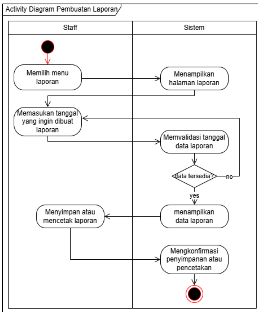
Gambar III.18 Activity Diagram Staff Membuat Laporan
