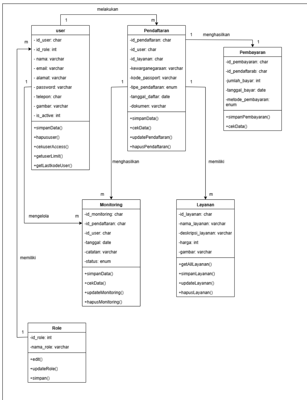
Gambar III.27 Class Diagram
