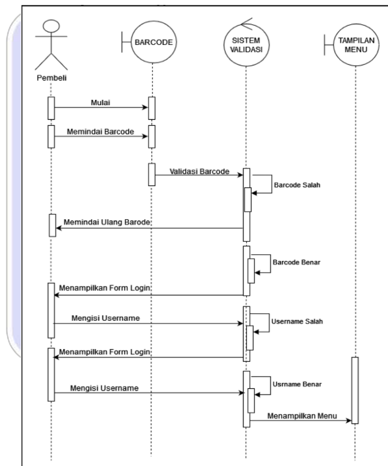
Gambar II.6 Contoh Sequence diagram
