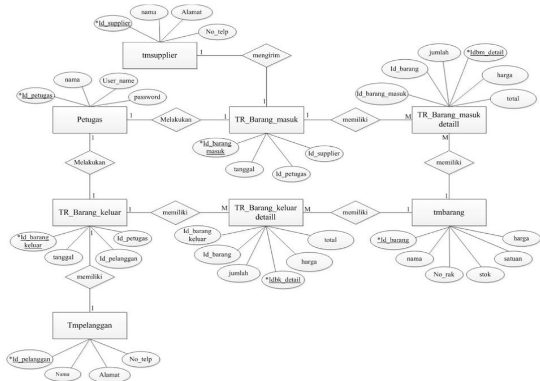
Gambar II.2 Contoh Entity Relationship Diagram (ERD)
