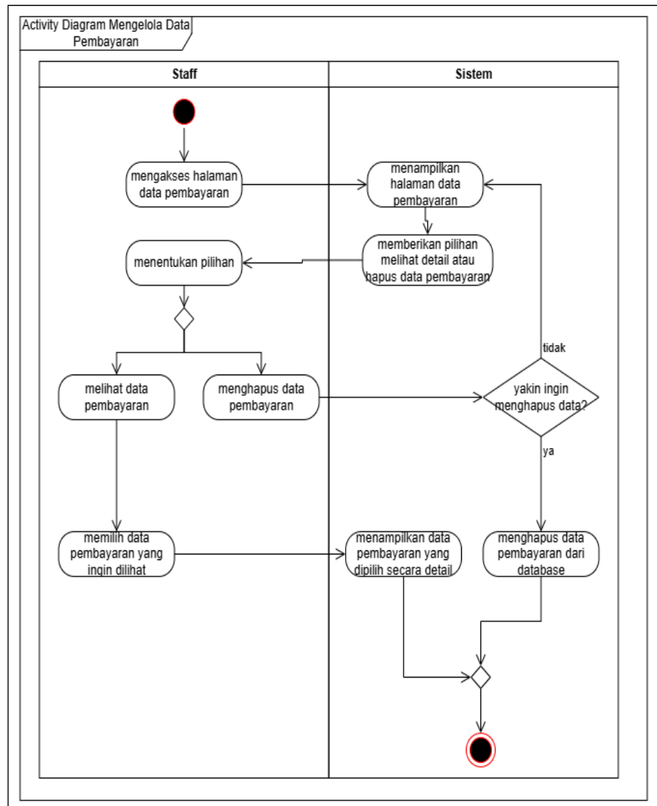
Gambar III.16 Activity Diagram Staff Mengelola Data Pembayaran
