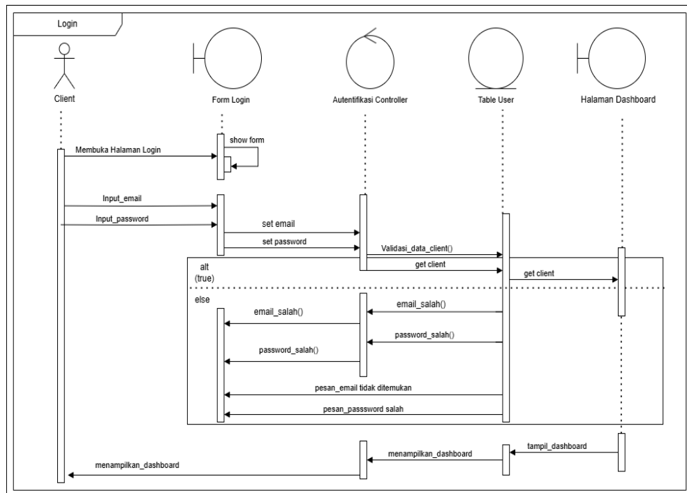
Gambar III.28 Sequence Diagram Client Melakukan Login
