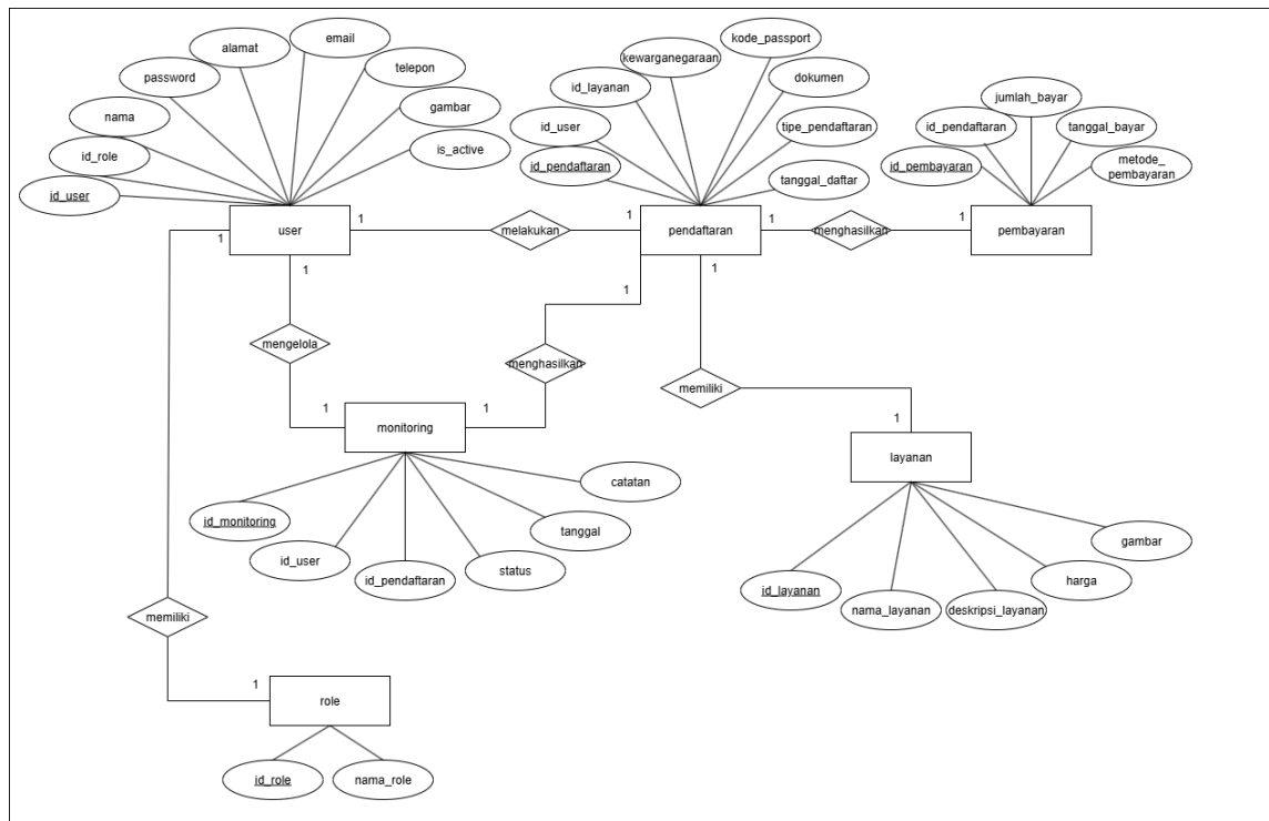
Gambar III.20 Entity Relationship Diagram
