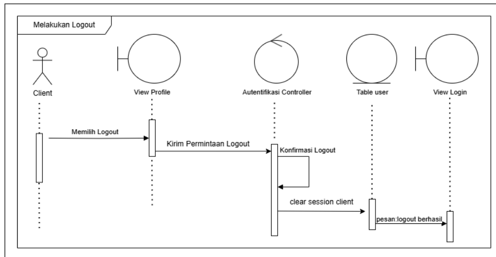
Gambar III.33 Sequence Diagram Client Melakukan Logout
