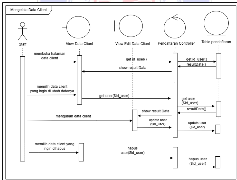
Gambar III.34 Sequence Diagram Staff Mengelola Data Client
