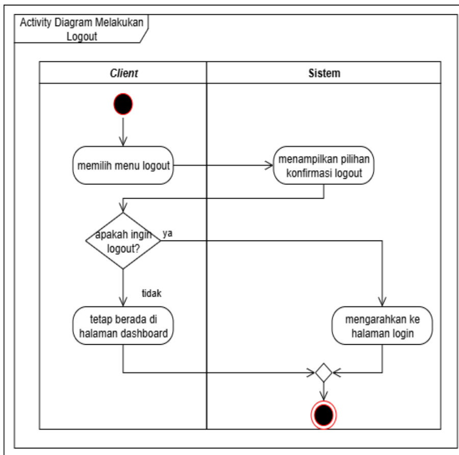
Gambar III.9 Activity Diagram Client Melakukan Logout
