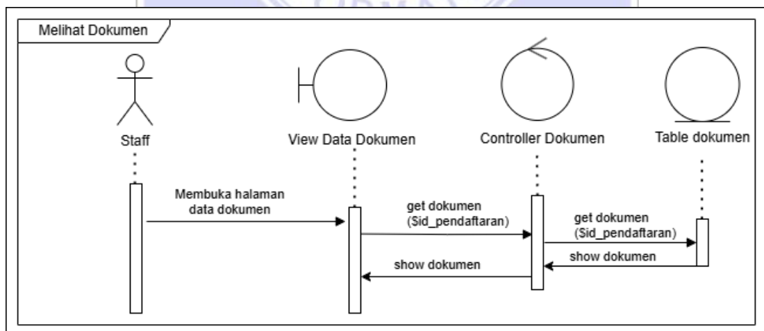
Gambar III.36 Sequence Diagram Staff Melihat Dokumen Client
