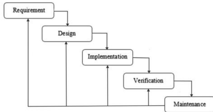
Gambar II.1 Metode Waterfall
